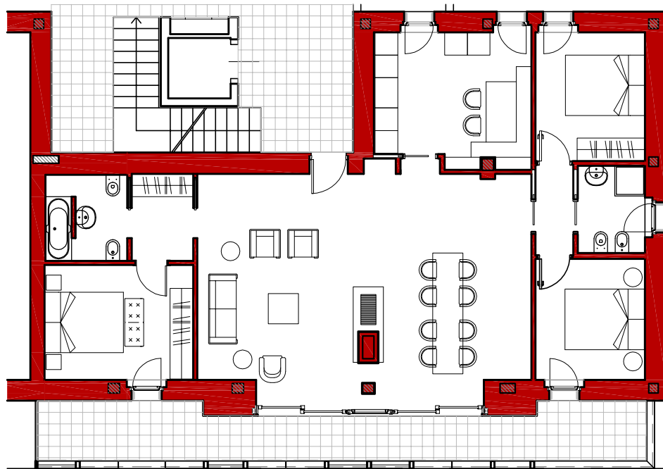
Piano Attico
